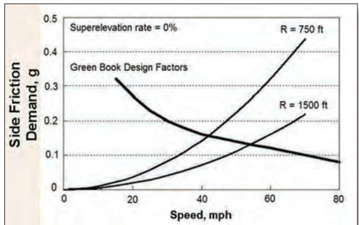
Relationship between curve speed and side friction demand for two radii
